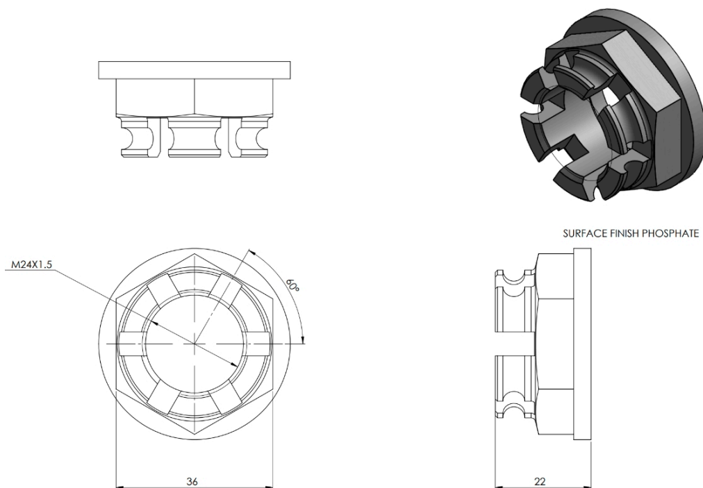
Technical Drawing: M24CNW
