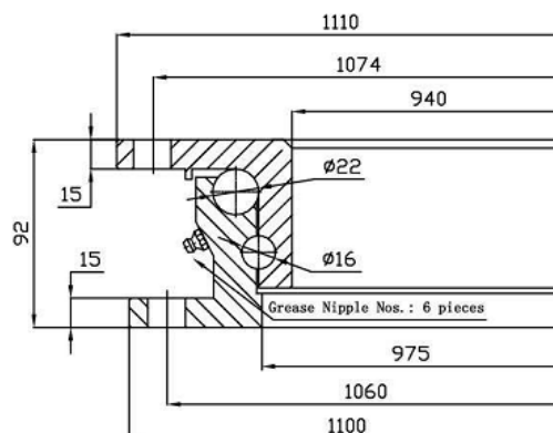
TL6-1100DT: Heights and Dimensions
