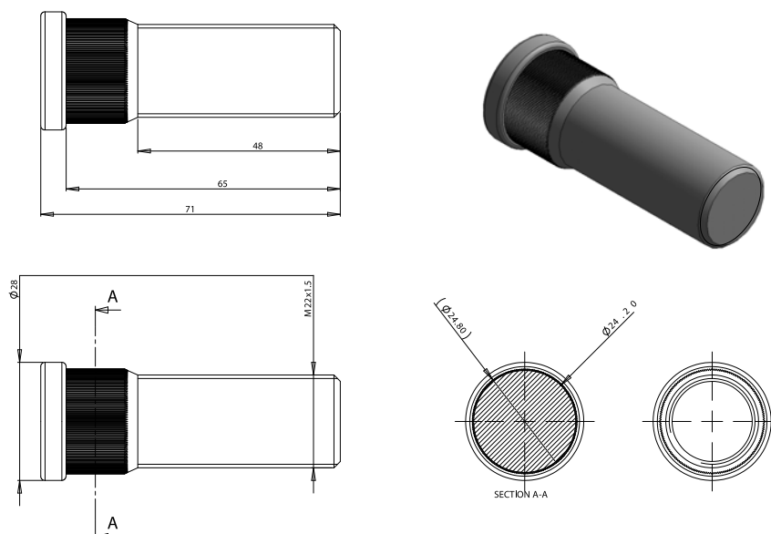
Technical Drawing: M22WS
