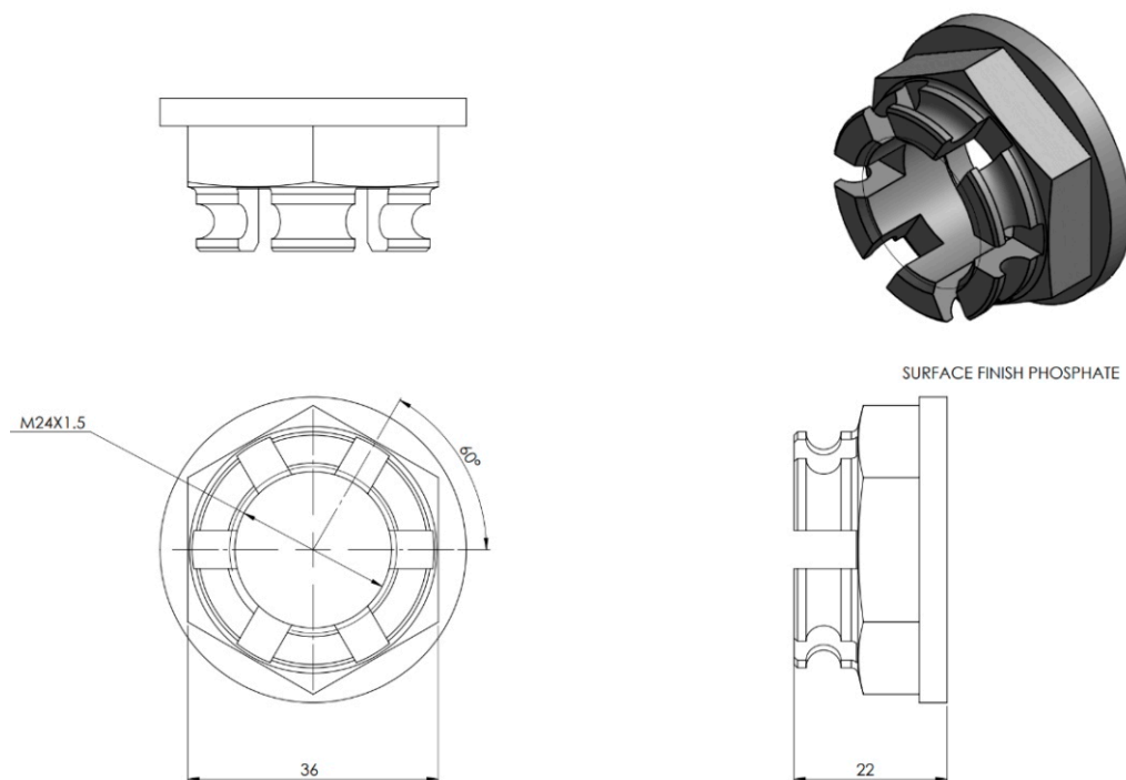
Technical Drawing: M24CNW
