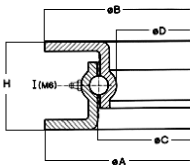
Turntables: Heights and Dimensions
