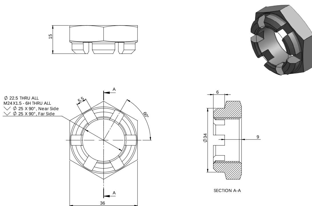
Technical Drawing: M24CN
